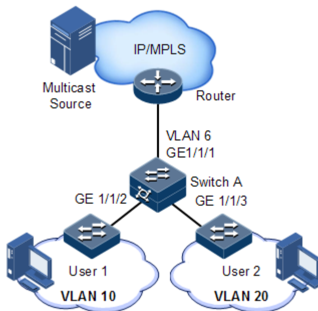
Figure 12-3 Multicast VLAN copy scenario
