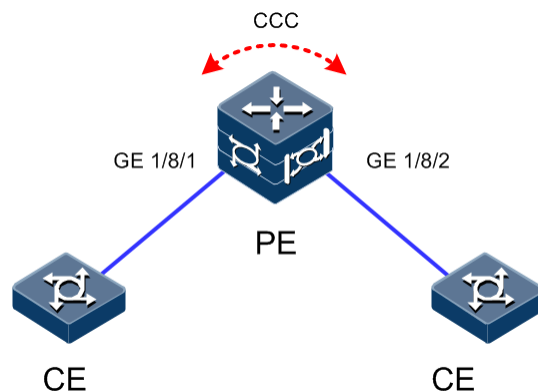
Figure 10-1 CCC local connection
