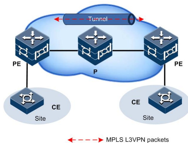
Figure 10-2 MPLS L3VPN network topology
