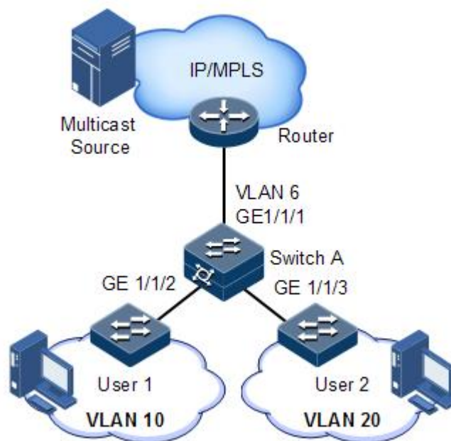
Figure 12-2 IGMP MVR application
