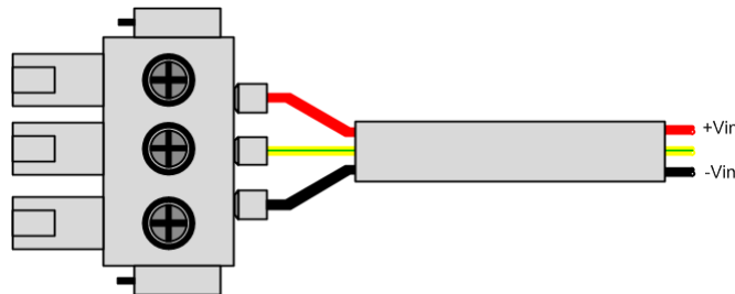
Figure 4-9 DC power cable
