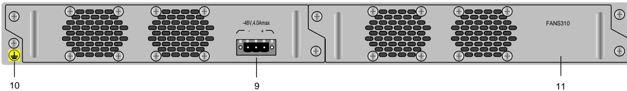
Figure 2-6 Rear appearance of the RAX721-T-XF single DC+FANS310 model
