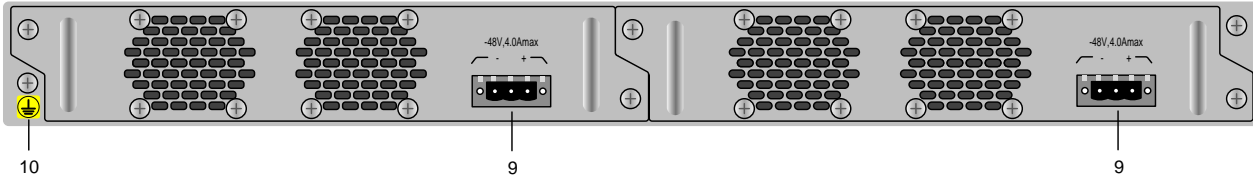
Figure 2-3 Rear appearance of the RAX721-T-XF dual DC model
