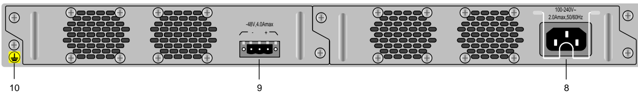
Figure 2-4 Rear appearance of the RAX721-T-XF AC + DC model
