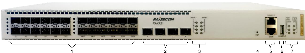
Figure 2-1 Front appearance of the RAX721-T-XF
