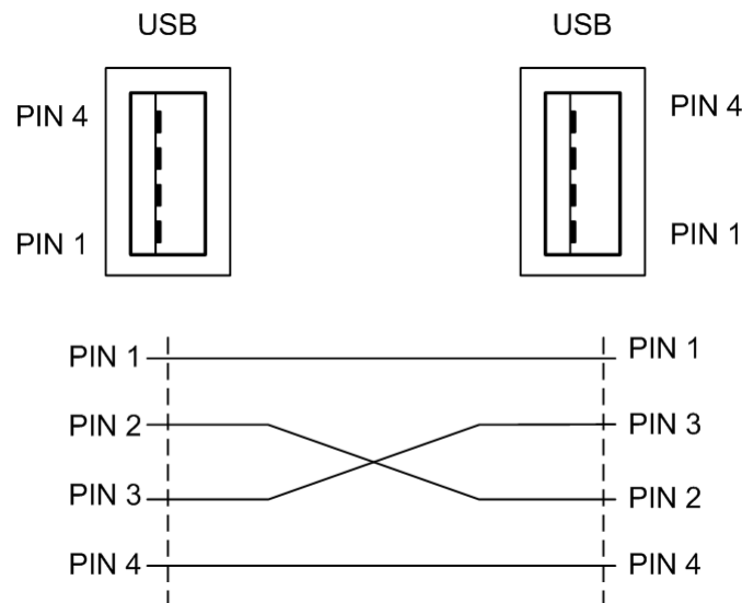
Figure 4-7 PINs and wiring
