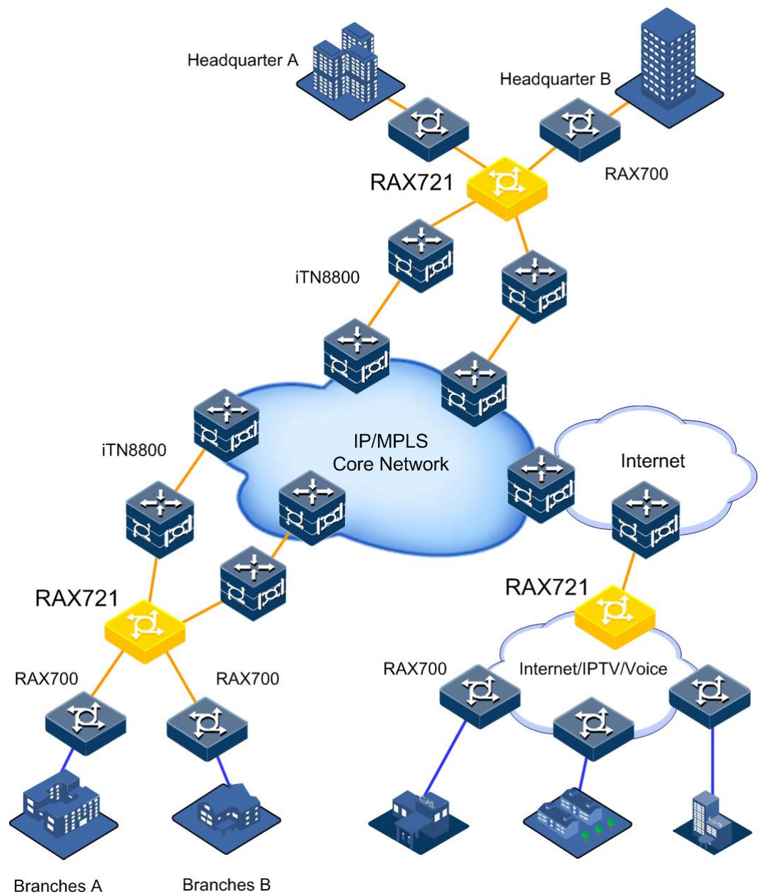
Figure 1-1 RAX721-T-XF networking
